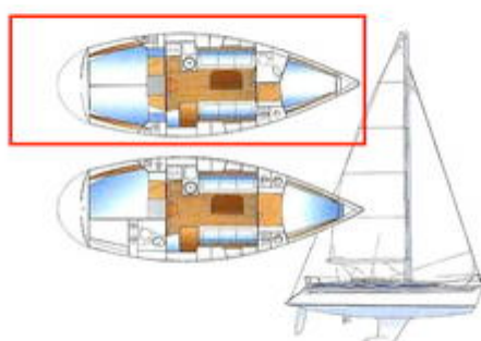
BAVARIA 34 (3 cabin)
