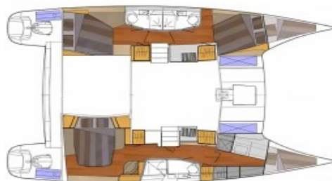
Fountaine Pajot Orana 44 Maestro Version
